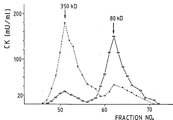
Fig. 2. Oligomeric state of mitochondrial creatine kinase in extracts from rat brain mitochondria as analyzed by gel chromatography. Brain mitochondria isolated in 0.25 M mannitol and 0.071 M sucrose were pretreated with 100 \mu\text{g} digitonin per mg. After centrifugation the mitochondria were resuspended in the same medium and 20 mM phosphate, 100 \mu\text{M} p -aminobenzamidine and 1.5% deoxycholate was added. The extract was chromatographed on a Superose 12 column. Elution profile of creatine kinase activity from an extract of untreated mitochondria (X), same extract after incubation with 3 M urea (◇). The activity of octamer and dimer was determined in the eluted fractions and is expressed as percent of the total activity which was eluted.
