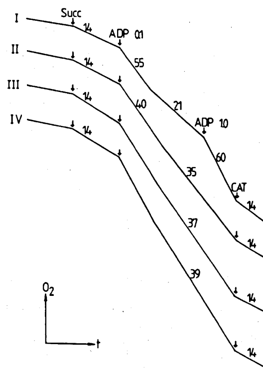
Fig. 4. Activation of state-3 respiration in brain mitochondria by creatine via internal creatine kinase. The oxygen consumption (nmol O 2 /min per mg) of isolated mitochondria from brain was determined in isolation medium containing 5 mM succinate, 5 \mu\text{M} rotenone, 5 mM phosphate and MgCl 2 . State 3 respiration was induced either by 0.1 mM ADP or 1.0 mM ADP (curve I), or by ADP regenerated by the reaction of mitochondrial creatine kinase in the presence of 25 mM creatine and 0.1 mM ADP, (curve II). Curves III and IV were obtained under the same conditions as curve II, but with mitochondria which were pretreated with 100 (III) or 300 \mu\text{g}/\text{mg} (IV) digitonin washed and resuspended in isolation medium. Carboxyatractylolide (CAT) 100 \mu\text{M} was added as indicated.
