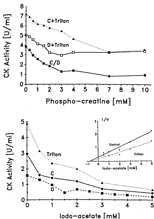
Fig. 6. Inhibition of mitochondrial creatine kinase by phosphocreatine or iodoacetate. The creatine kinase activity of brain mitochondria either intact (C) or after treatment with 100 \mu\text{g}/\text{mg} of digitonin (D) was determined in isotonic medium and after addition of 1% Triton X-100 both containing 5 mM succinate and 2 mM phosphate and \text{MgCl}_2 and 1 \mu\text{M} oligomycin. The enzyme reaction which was measured from creatine and ATP was inhibited either by increasing concentrations of creatine phosphate (Panel A) or iodoacetate (Panel B) as indicated. The data from Fig. 6B (Triton and C) were used for the Dixon plot shown as inset in the same figure.
