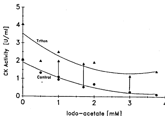
Fig. 8. Protection of latent Mi-CK activity against iodoacetate inhibition. Suspension of intact mitochondria were pre-incubated with increasing concentrations of iodoacetate. The activity of creatine kinase was determined in aliquots of the pretreated mitochondria in the absence of inhibitor either under isotonic conditions (Control) as in Fig. 6B or after subsequent addition of 1% Triton (Triton) to the same samples resulting in the liberation of uninhibited activity.
