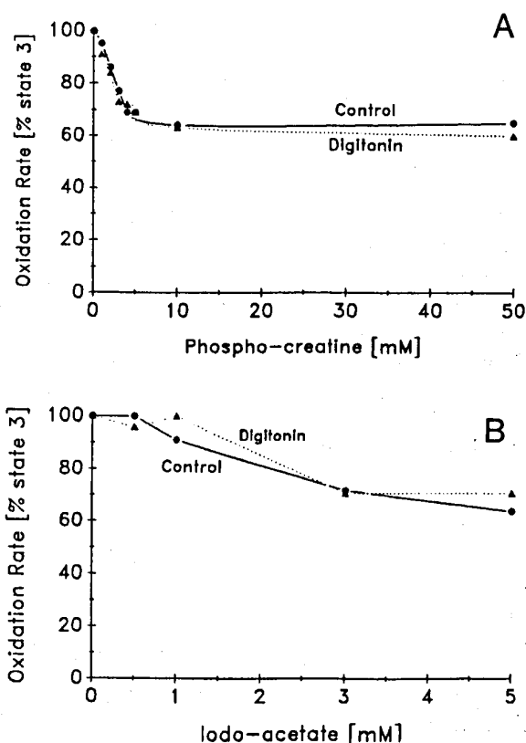
Fig. 7 Inhibition of creatine stimulated state-3 oxidation by phosphocreatine or iodoacetate. The oxygen consumption (nmol \text{O}_2/\text{min} per mg) of brain mitochondria was determined in isolation medium containing 5 mM succinate, 5 \mu\text{M} rotenone, 5 mM phosphate and \text{MgCl}_2 . State 3 respiration was induced by the reaction of mitochondrial creatine kinase in the presence of 20 mM creatine and 0.1 mM ADP. The oxidation rate after addition of either phosphocreatine (Panel A) or iodoacetate (Panel B) is expressed as % of the maximal state 3 activity in the presence of 1 mM ADP. The latter state 3 activity was not effected by iodo acetate up to 5 mM. The same experiments were performed with mitochondria which were pretreated with 100 \mu\text{g}/\text{mg} digitonin, washed and resuspended in isolation medium. For a control these mitochondrial preparations were incubated with 100 \mu\text{M} carboxyatractyloside which fully blocked oxidative phosphorylation (see also Fig. 4).
